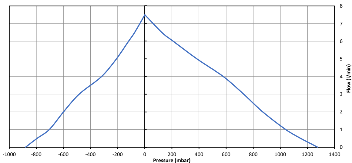
Flow / Pressure characteristic
